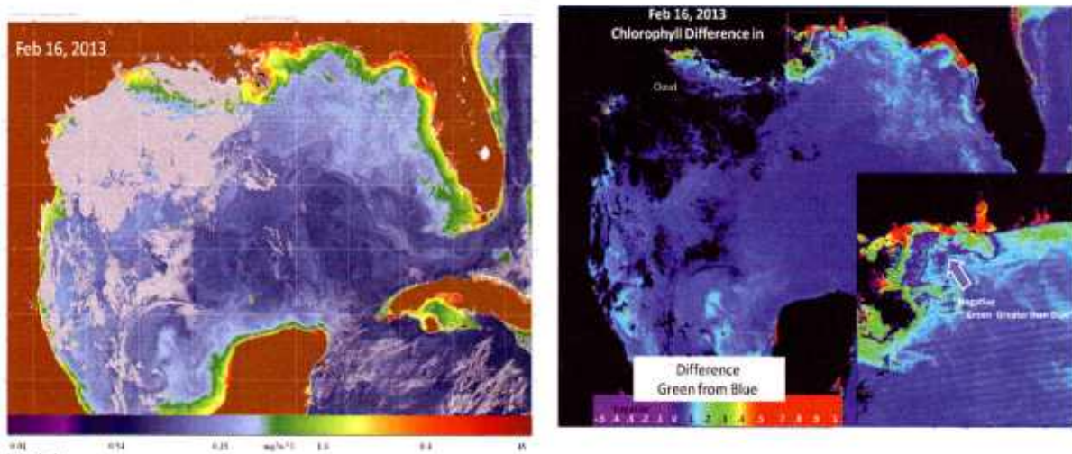
Figure 4. A. SNPP chlorophyll product for Feb 16, 2013 processed using blue and green gains. B. The difference in chlorophyll (mg/m 3 ) between that processing using the values from the green gain processing minus the blue gain. The subset is the Mississippi Delta coastal area. The scale shows minimal difference (0) in mg/m 3 in dark blue difference represented for open ocean waters. The purple areas indicate negative chlorophyll difference, where the Blue gain produced high chlorophyll than the Green gain. The red show areas of increased chlorophyll with the green gain. (Color copies http://parrotfish.ssc.usm.edu/~owx/pubs )
