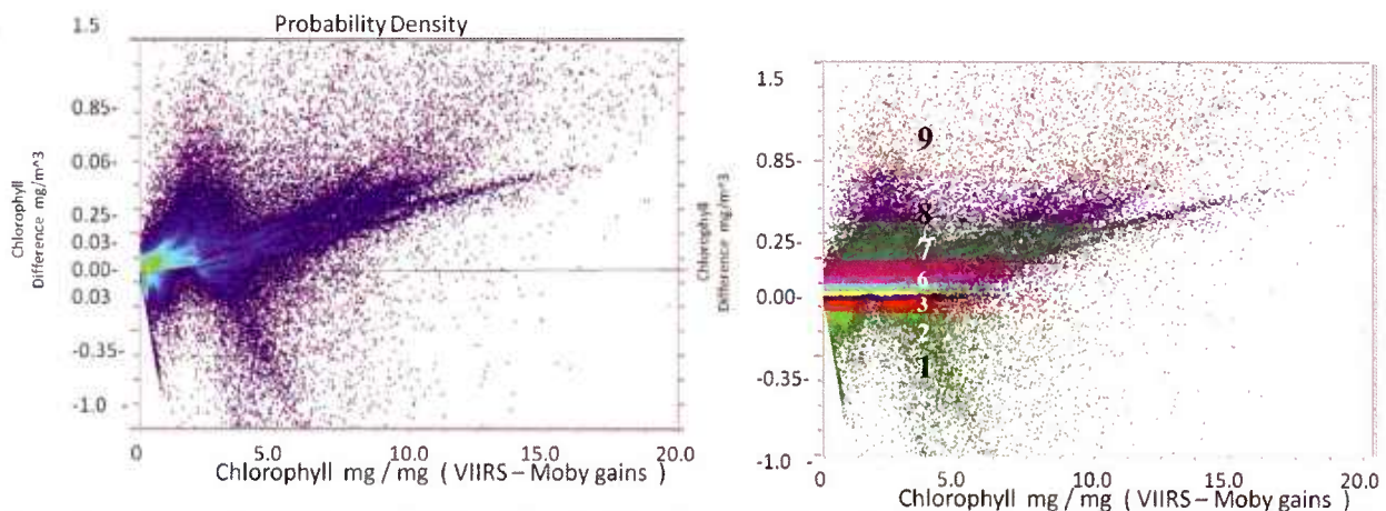
Figure 7 – A. Scatterplot of difference of chlorophyll using blue and green gains is related to the chlorophyll concentration derived from the Blue gain for Feb 16. B. Regional Difference color map
