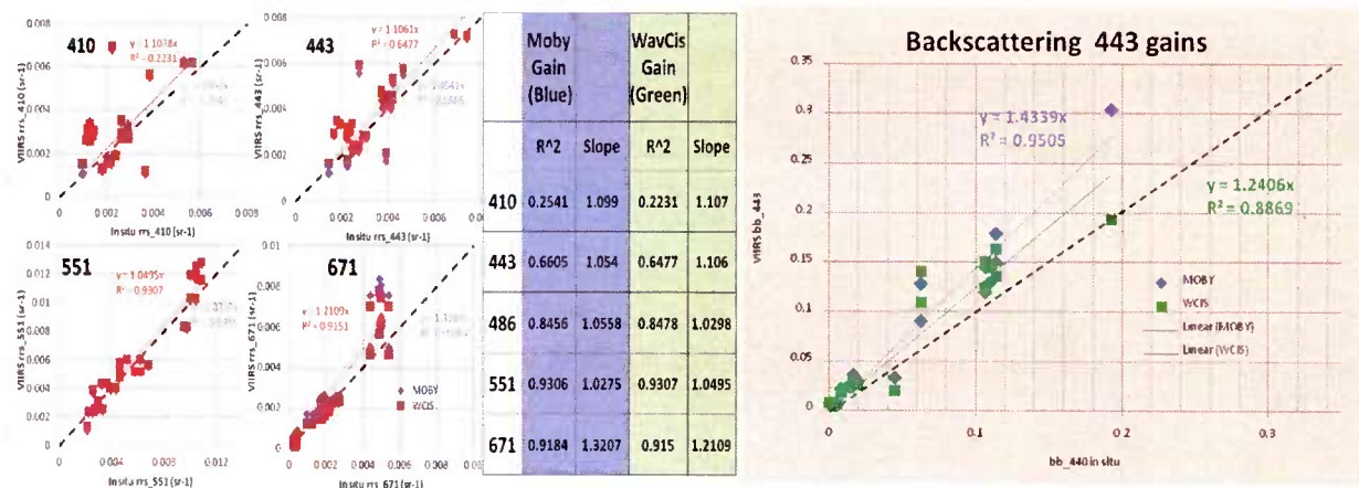
Figure 10 A) Scatterplots of insitu Remote Sensing Reflectance (RRS) with VIIRS RRS using the blue and green gain for 4 channels. Table shows the regression ( R^2 ) and slope. The green gain shows slope closer to the 1. B) In-situ backscatter 443 and VIIRS bb443 products using the blue and greens gains is illustrated. The slope of the green gain is closer to the 1 to 1 line.
