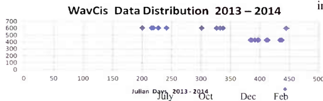
Figure 1- The green water gains were computed from the WaveCis AERONET site in the Northern Gulf of Mexico from July 2013 to Feb 2014 and included 21 points after constraints were applied ( see Bowers et al 2014) 7 .
