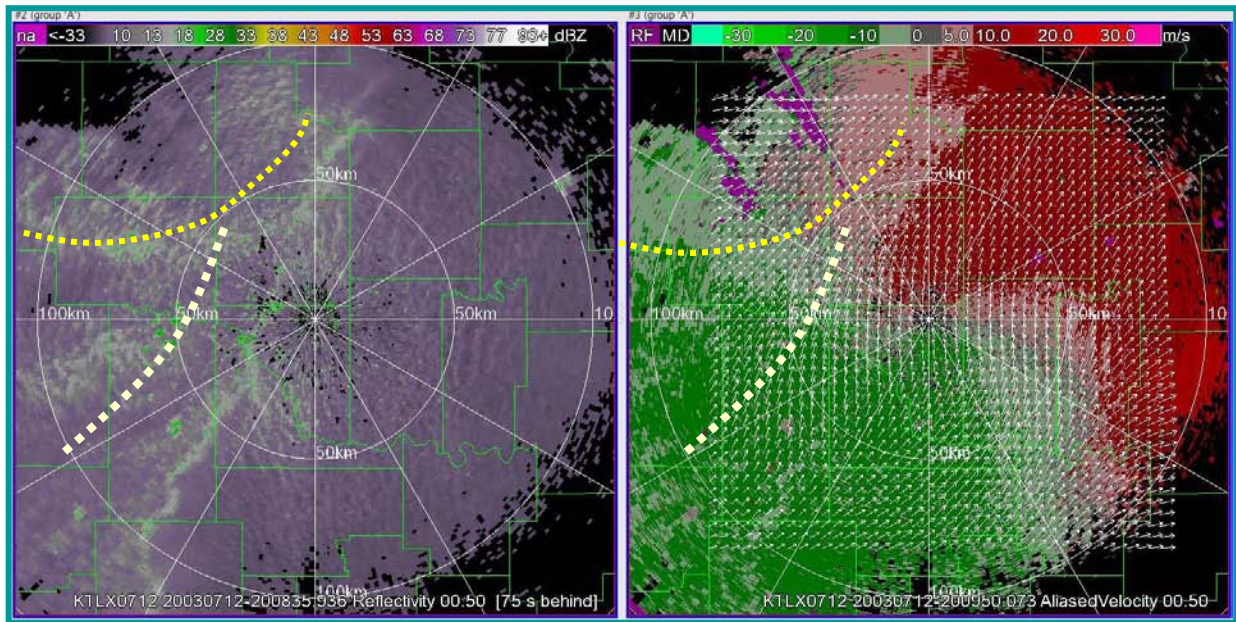
Fig. 2. KTLX observed reflectivity (left panel) and radial-wind (color field, right panel) overlaid with the retrieved wind vectors on 0.5^\circ elevation at 20:09 UTC on July 12, 2003. The yellow and white dashed lines mark the boundaries of wind shear and convergence.
