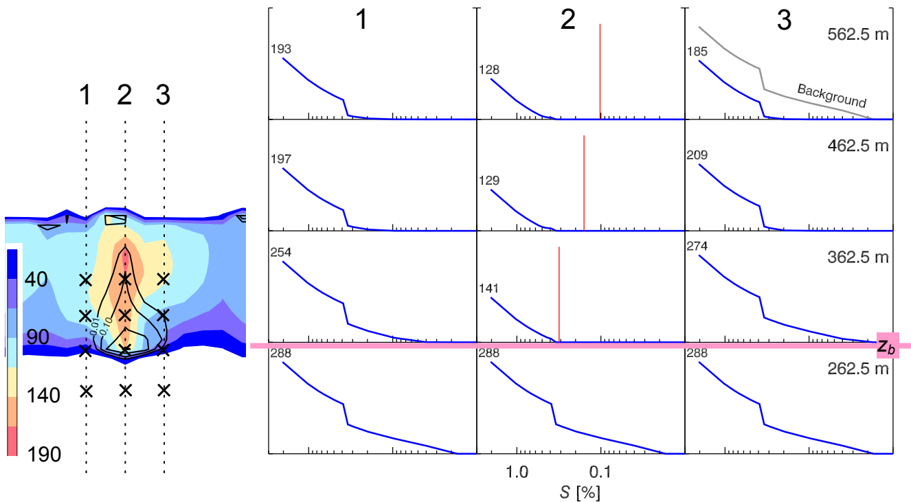
Figure 1. A vertical cross section of supersaturation (black contours) and droplet concentration (filled contours, units of [cm^{-3}] ) in a supersaturated updraft region. Cloud depth is approximately 350 m. Panels are CCN spectra in and adjacent to a supersaturated updraft core, taken from model grid points indicated by the “x” points in the left hand vertical cross section. Numbers indicate total CCN at each point, and red bars represent grid point supersaturation (if over 0.01%).
