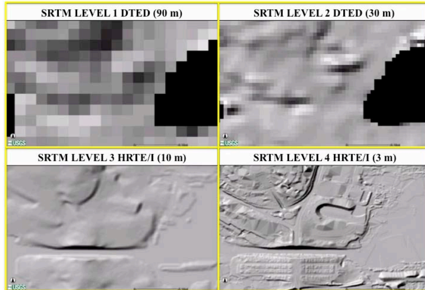
Figure 16. SRTM elevation data resolutions: DTED® and HRTE/I.
