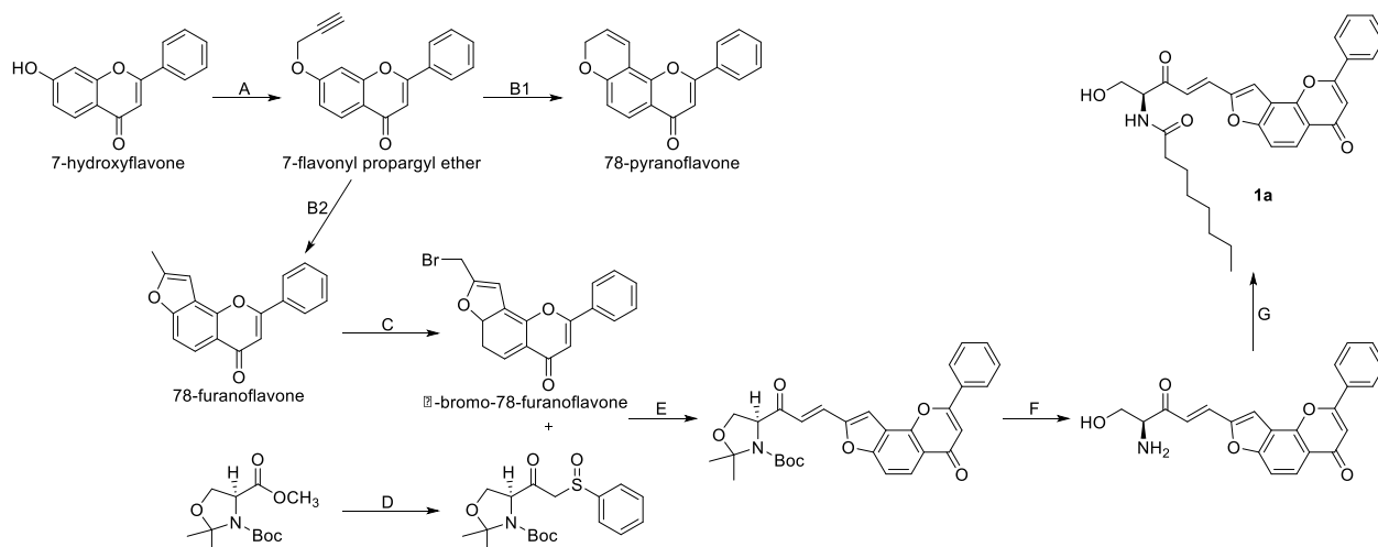
Figure 4. Synthetic route for flavonyl-modified ceramide analogs. Step A) propargyl
