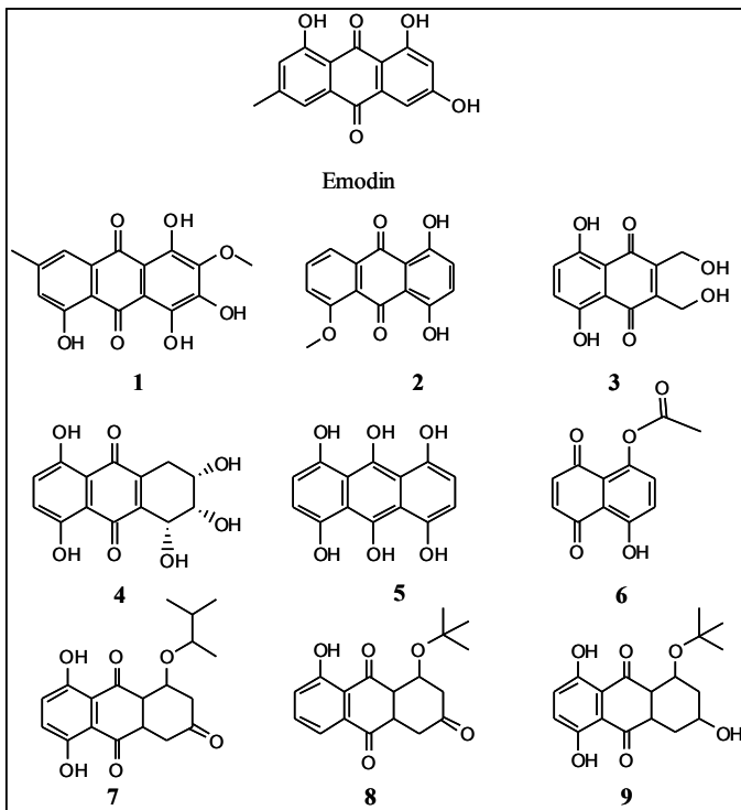
Figure 14: Structure of emodin and compounds 1 to 9 investigated for inhibition of Pim 1 kinase.
