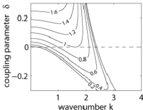
Figure 1: Theoretical growth rate (normalized by the maximum growth rate for the uncoupled Eady problem) as a function of the wavenumber k and a coupling parameter \delta . For winds from warm to cold, \delta > 0 while for winds from cold to warm \delta < 0 . If there is no active coupling between SST and surface winds, \delta = 0 . Typical values of \delta range from 0.01 for strong separated western boundary currents to 0.25 for shallow shelf break fronts or low-latitude zonal currents.
