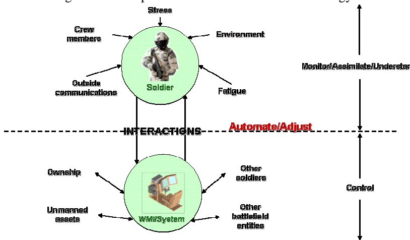
Figure 4: Adaptive Automation
