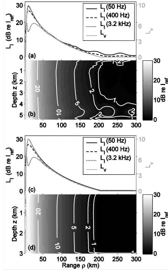
Figure 1: Predicted noise spectral level in the North Atlantic (a) and (b) and the Bay of Bengal (c) and (d). (a) and (c) show the level as a function of range at a depth of 200 m for 50, 400 and 3200 Hz frequencies. L_V(\rho) = 10 \log(V(\rho)/V_{ref}) if plotted for comparison where V_{ref} = 5 m/s. L_V = 0 is equivalent to V = 5 m/s and L_V = 10 is equivalent to V = 50 m/s. (b) and (d) show the spectral level as a function of range and depth at 50 Hz. In both waveguide environments the noise level closely follows the local wind speed. In the North Atlantic there is a convergence zone structure corresponding to sound that propagates from the hurricane's eye wall via refraction. Note the convergence zone near the surface at a range of 257 km and the ray vertex depth of 4.7 km.
