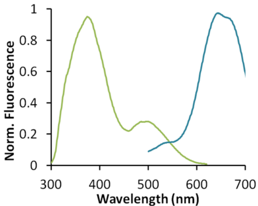
Fig. 6 Normalized fluorescence excitation and emission spectrum of DNase 1-AuNCs synthesized with 0.5-mM HAuCl 4
