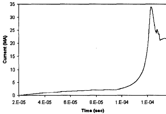
Fig. 6. Current from 1.4 m Ranchero test.
