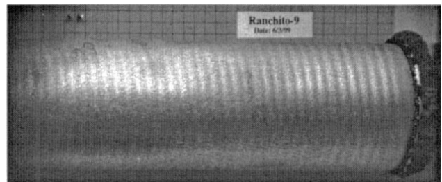
Figure 5. Rotating mirror camera record of 1.4 m armature expanded to the approximate final diameter for use in a Ranchero generator. Only about 2/3 of the armature is shown in this frame. The remainder of the armature was seen with a second camera. The grid pattern is 25.4 mm per line.
