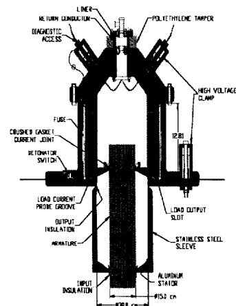
Figure 2. Cutaway drawing of system in Fig. 1.
