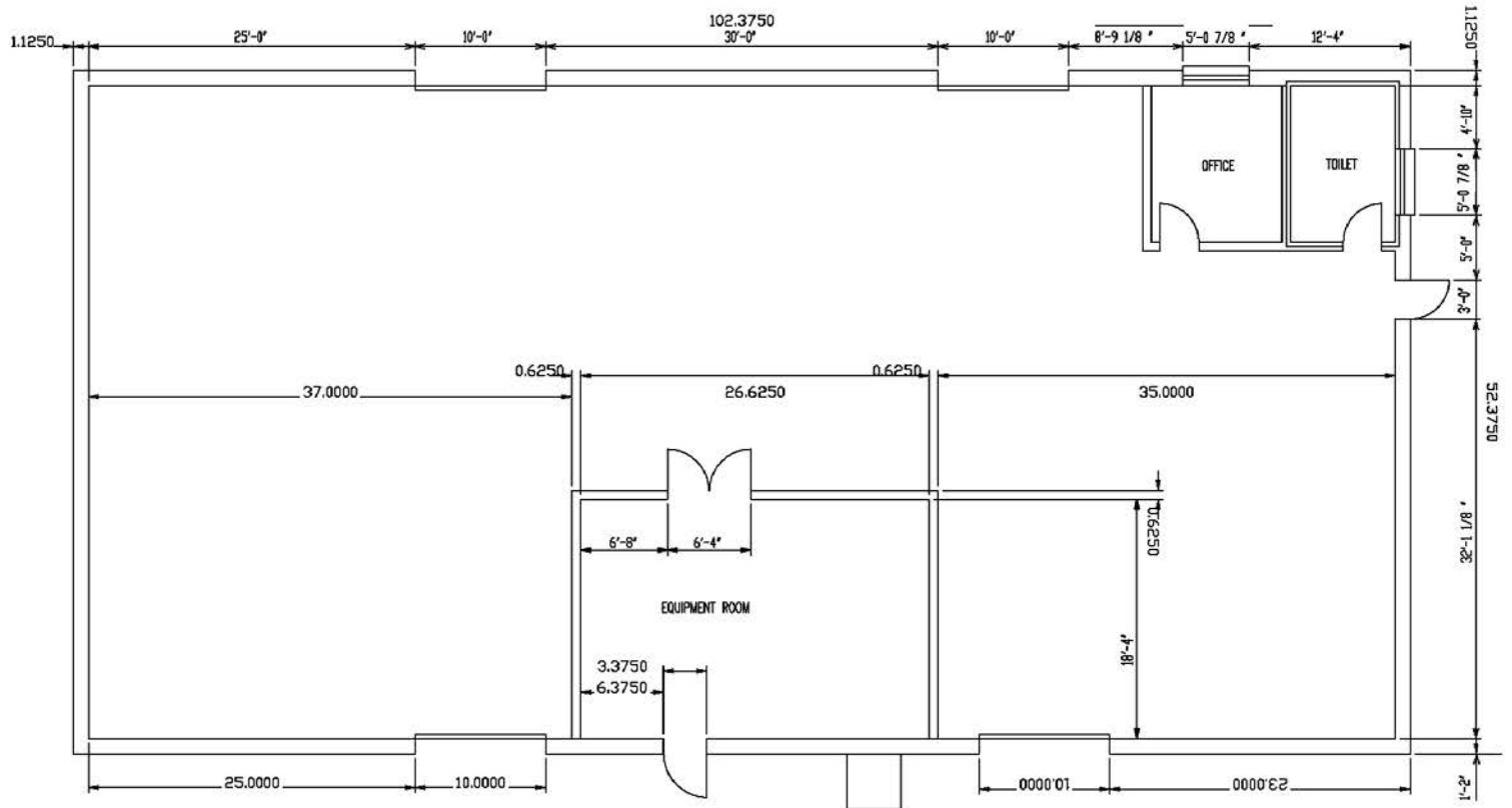
BUILDING 88315 DRAWN: 9 AUG. 00 SCALE: 1/8" = 1'-0"
