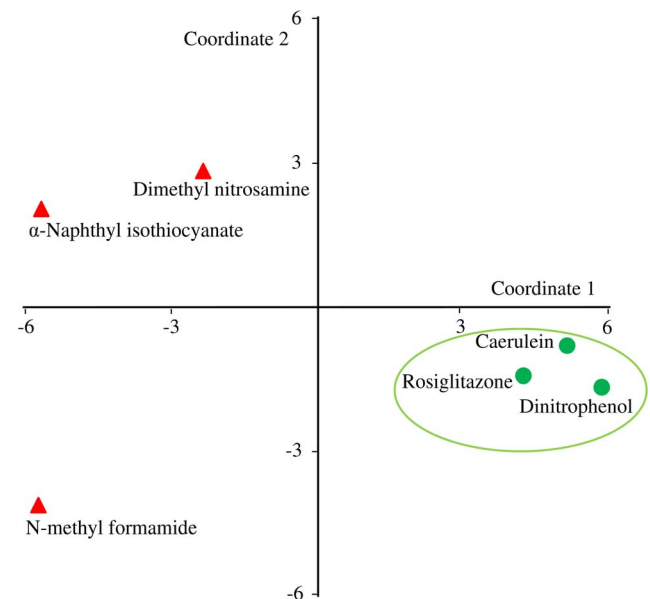
Figure 11. Analysis of exposures in GSE5509 using the general liver injury gene signature. Multidimensional scaling (MDS) plot of six chemical exposures in GSE5509 using the general liver injury gene signature. This figure shows the ability of the genes in the general liver injury signature to separate toxicants from non-toxicants. Rosiglitazone, caerulein, and di-nitro phenol, the non-toxic compounds in this set are marked in green circles. \alpha -Naphthyl-isothiocyanate, dimethyl nitrosamine, and N-methyl formamide are the toxic compounds in this set, and they are marked with red triangles. In the MDS plot, the non-toxic compounds clustered separately from the toxic compounds. We have highlighted the non-toxic compounds within a green circle. doi:10.1371/journal.pone.0107230.g011
