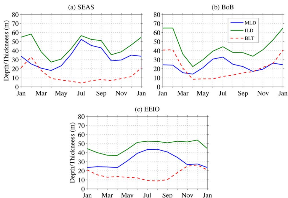
Figure 5. The seasonal evolution of the MLD (blue), ILD (green), and BLT (dashed red) for the (a) SEAS, (b) BoB, and (c) EEIO from Argo. January is shown twice to complete the seasonal cycle. BLT in the above figure is computed as the difference between the ILD and MLD averaged from 2005 to 2012 (ILD-MLD).
