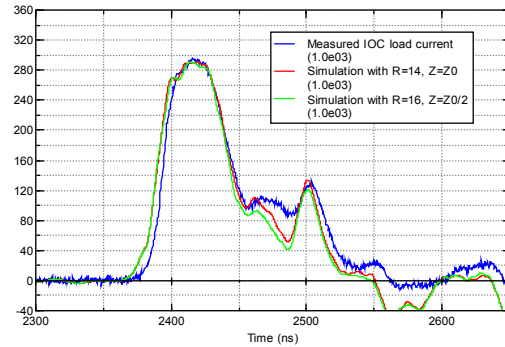
Figure 7. Measured and simulated load currents for shot #0628 (7-cm AK gap).
