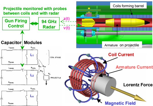
Figure 2. System components of induction coilgun.
