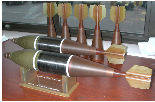
Figure 3. XM934 EM coilgun projectiles and tail kits.
