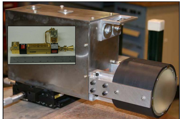
Figure 4. Coilgun projectile tracking radar system.
