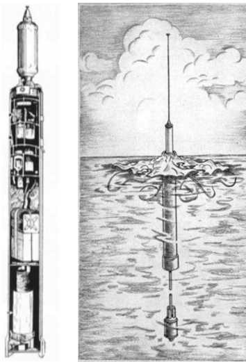
Cut-Away Deployed
