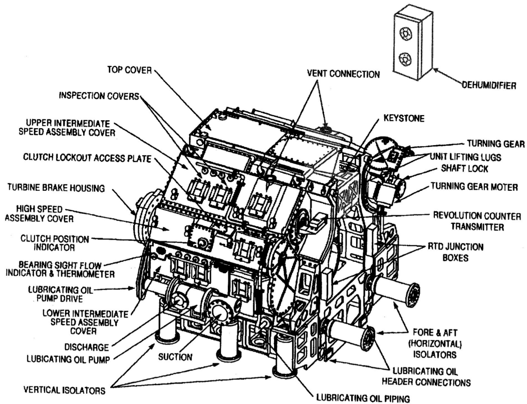
Figure 11: DDG 106 Propulsion Reduction Gear Arrangement, Port Gear, Isometric View (Hellman 2013) - Unclassified
