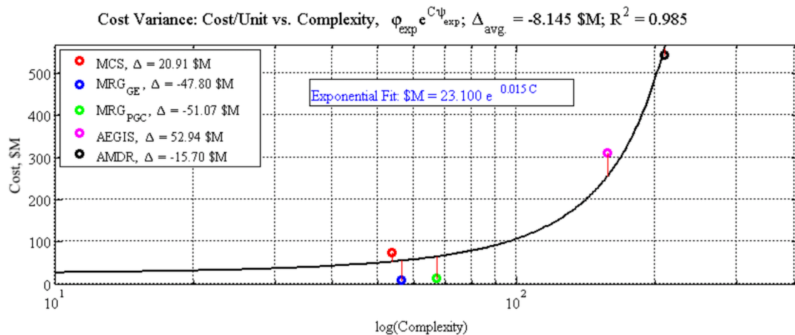
Figure 19: Unit Cost vs. Complexity, Exponential Fit: \$M = 23.1e^{0.015C}
