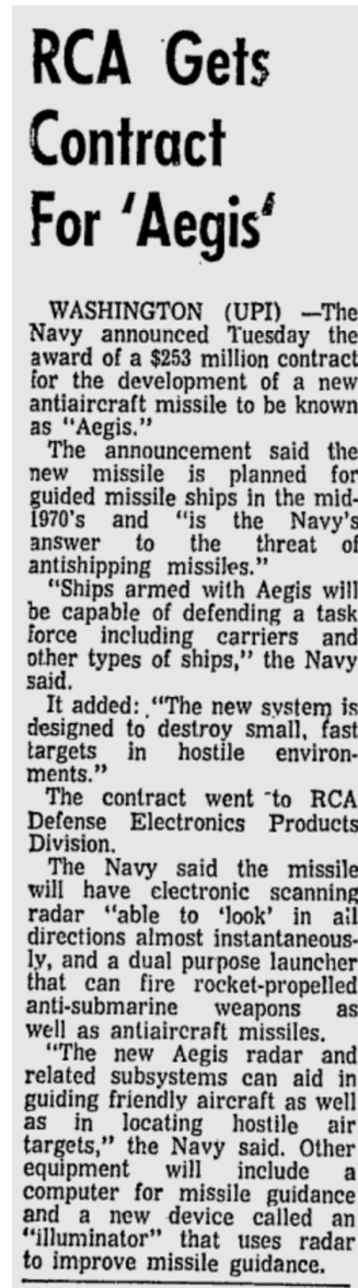
Figure 15: RCA's 1969 Contract Initiation
