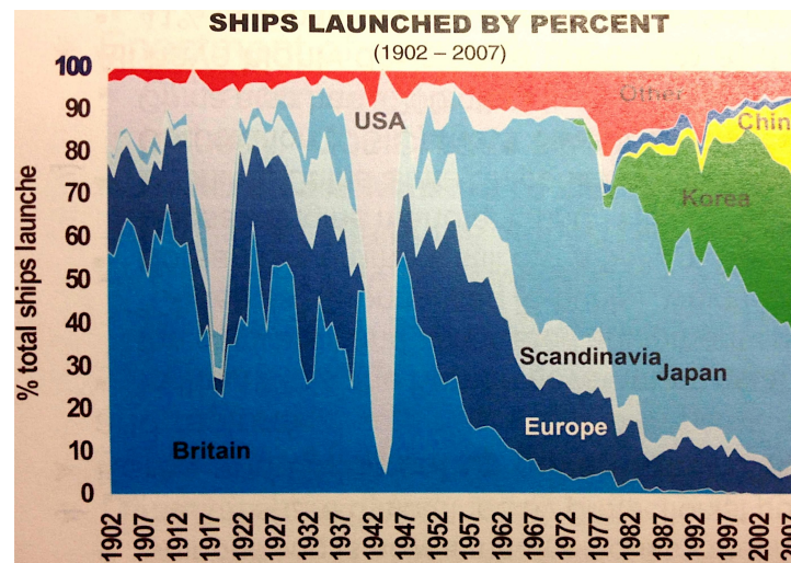
Figure 23: Worldwide Shipbuilding Market Share (Harris 2013)
