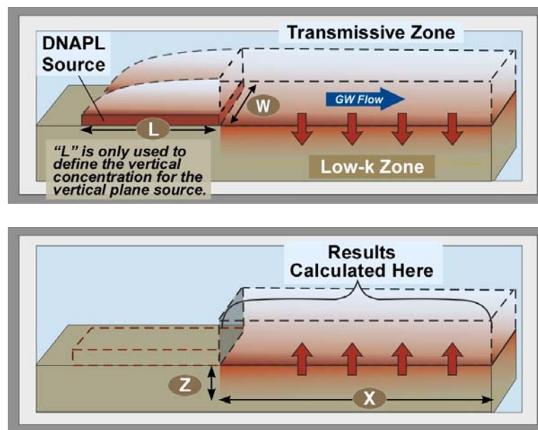
Figure A.2.7.1. The two-layer scenario conceptual model: Top) Active Source, Bottom) Depleted Source
