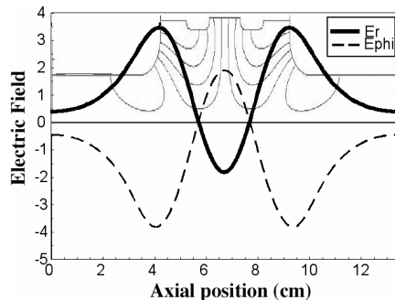
Figure 5 Field pattern of the TE_{113} -like hybrid mode of the magnicon output cavity, from calculations done by V.P. Yakovlev using the code CLANS2.
