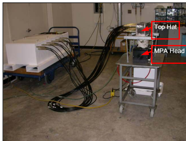
Figure 9. Offline test facility includes the actual flash lamp load.
