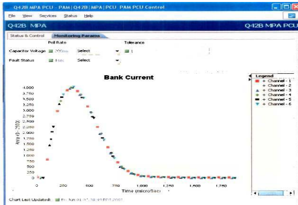
Figure 11. Current waveforms for all 6 lamp pair currents are displayed under the Monitor Parameters Tab.
