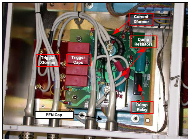
Figure 8. PFN Assembly includes Trigger Board, Trigger Transformer, and Capacitor.
