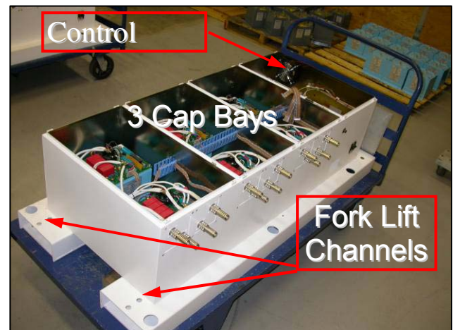
Figure 6. PCU Enclosure with the 4 access covers removed.
