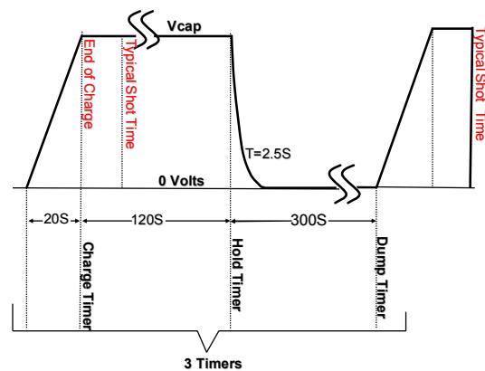
Figure 4. Capacitor Charging Voltage profile
