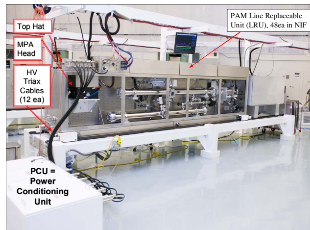
Figure 1. The PCU provides pulsed electrical power to the Multi Pass Amplifier within the Pre-amplifier Laser System.
