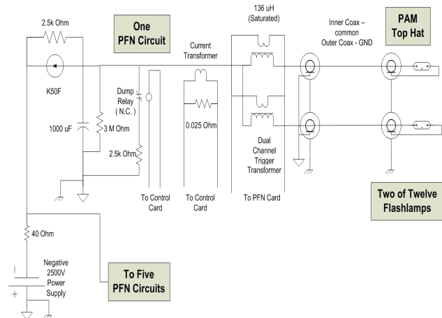
Figure 2. Simplified schematic of the PFN circuit driving a lamp pair.
