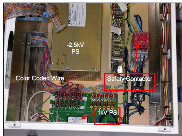
Figure 7. PWR Deck (located below control deck)
