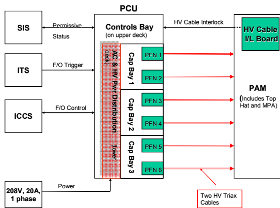
Figure 3. System Block Diagram of the PCU
