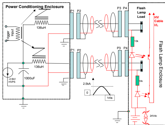
Figure 5. HV Cable Interlock Circuit shown for a lamp pair.
