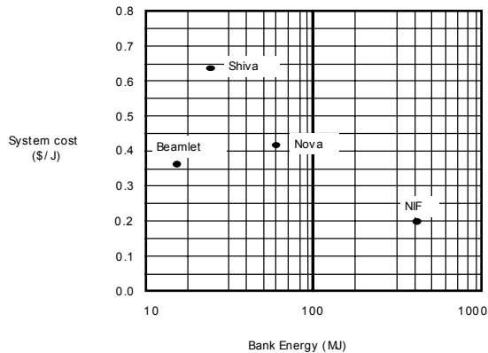
Figure 2. Per unit cost of stored energy for LLNL flashlamp drivers (in today’s dollars).
