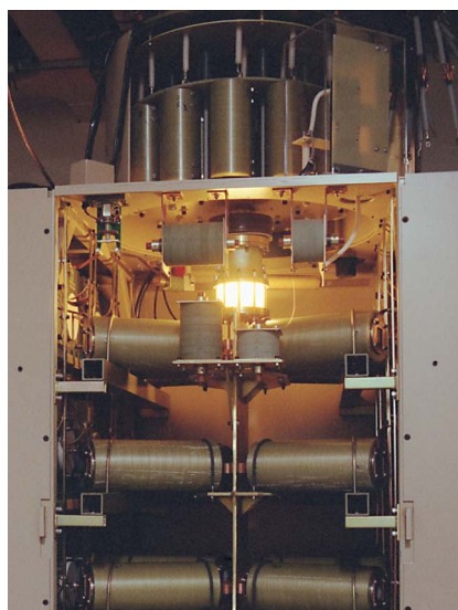
Figure 4. MESM discharge. Damping elements are visible below the switch. Ballast inductors are located above the switch in the “top hat.”
