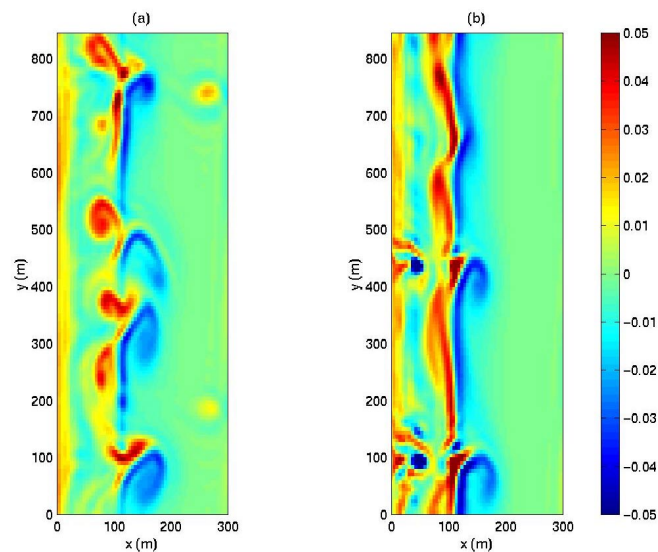
Figure 1: Snapshots of vorticity for shear instabilities on a barred beach with low frictional dissipation ( c_f=0.004 ) (a) neglecting and (b) including wave-current interaction.
