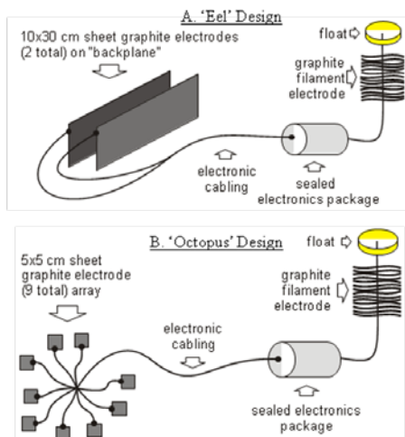
Figure 2. Schematic of the ‘Eel’ and ‘Octopus’ MFC system designed to take bacterial samples. Fig. 2A. ‘Eel’ design, 10x30 cm sheet graphite electrodes (2 total) on redwood backplane attached to electronic cabling. Fig. 2B. ‘Octopus’ design, 5x5 cm attached to electronic cabling. In both scenarios the sealed electronics package lies directly on the ocean sediment. The graphite filament electrode is suspended in the marine water column to a float.
