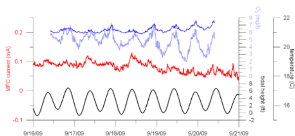
Figure 5. Dissolved oxygen and anode current near the bottom at in sediment with 2% total organic carbon (30% silts and clays). Power is shown relative to tidal height, oxygen (mg/L), and temperature (°C).
