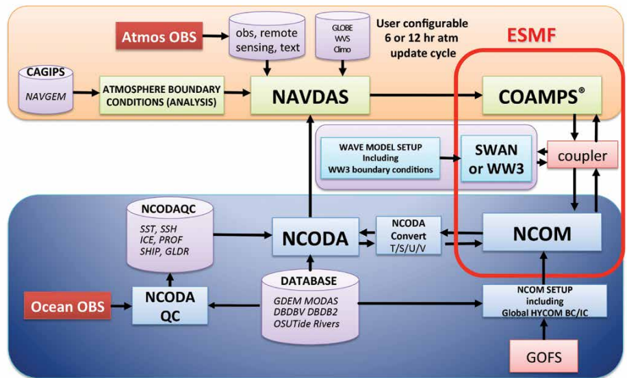
Figure 2. Flow diagram of the Coupled Ocean/Atmosphere Mesoscale Prediction System (COAMPS ® ) in its atmosphere-ocean-waves configuration. The atmosphere core model highlighted in orange, the ocean core model in blue, and the wave core model in purple.
