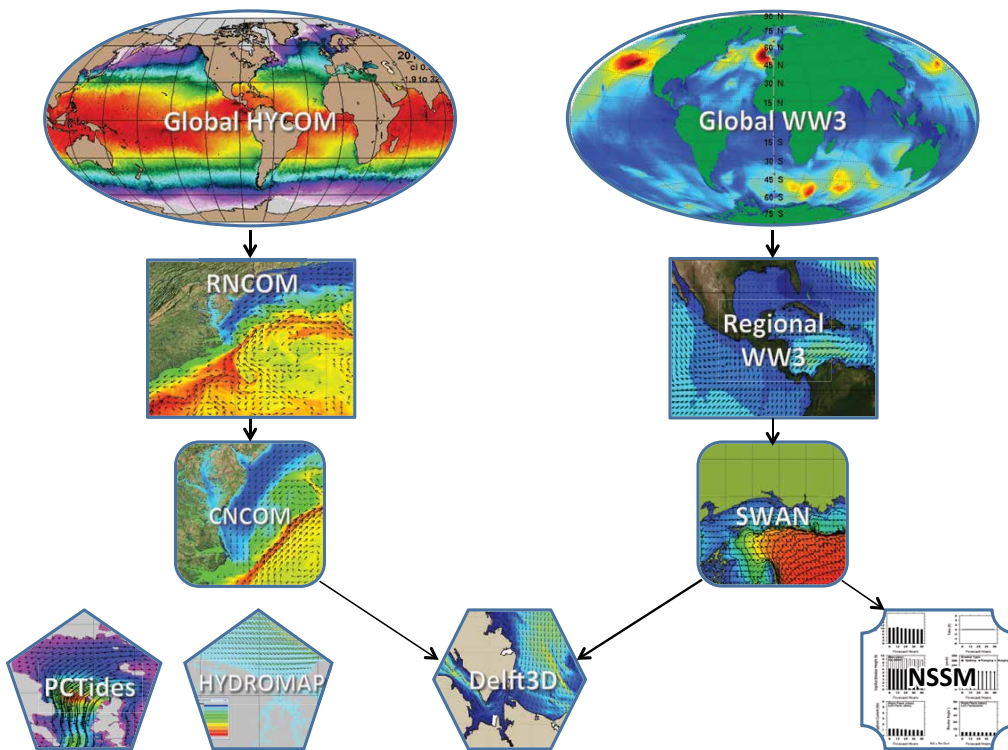
Navy Suite of Operational Circulation, Wave, Tide, and Surfzone Models
