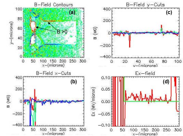
Figure 3. (a) Contours of the magnetic field in the nail head and wire body, (b) B-field in cuts 5 and 10 and 15 \mu\text{m} below the centerline, (c) vertical B-field cut at x = 120 \mu\text{m} , and (d) E-field along the centerline.
