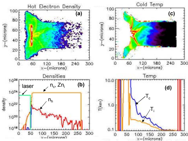
Figure 2. Conditions at 940 \text{ fs} in the Cu wire. (a) hot electron density contours, (b) hot electron density, n_h(x,y) on the centerline, (c) cold background temperatures T_c(x,y) , and (d) T_c and T_i (ion temperature) cuts at y = 50 \mu\text{m} .
