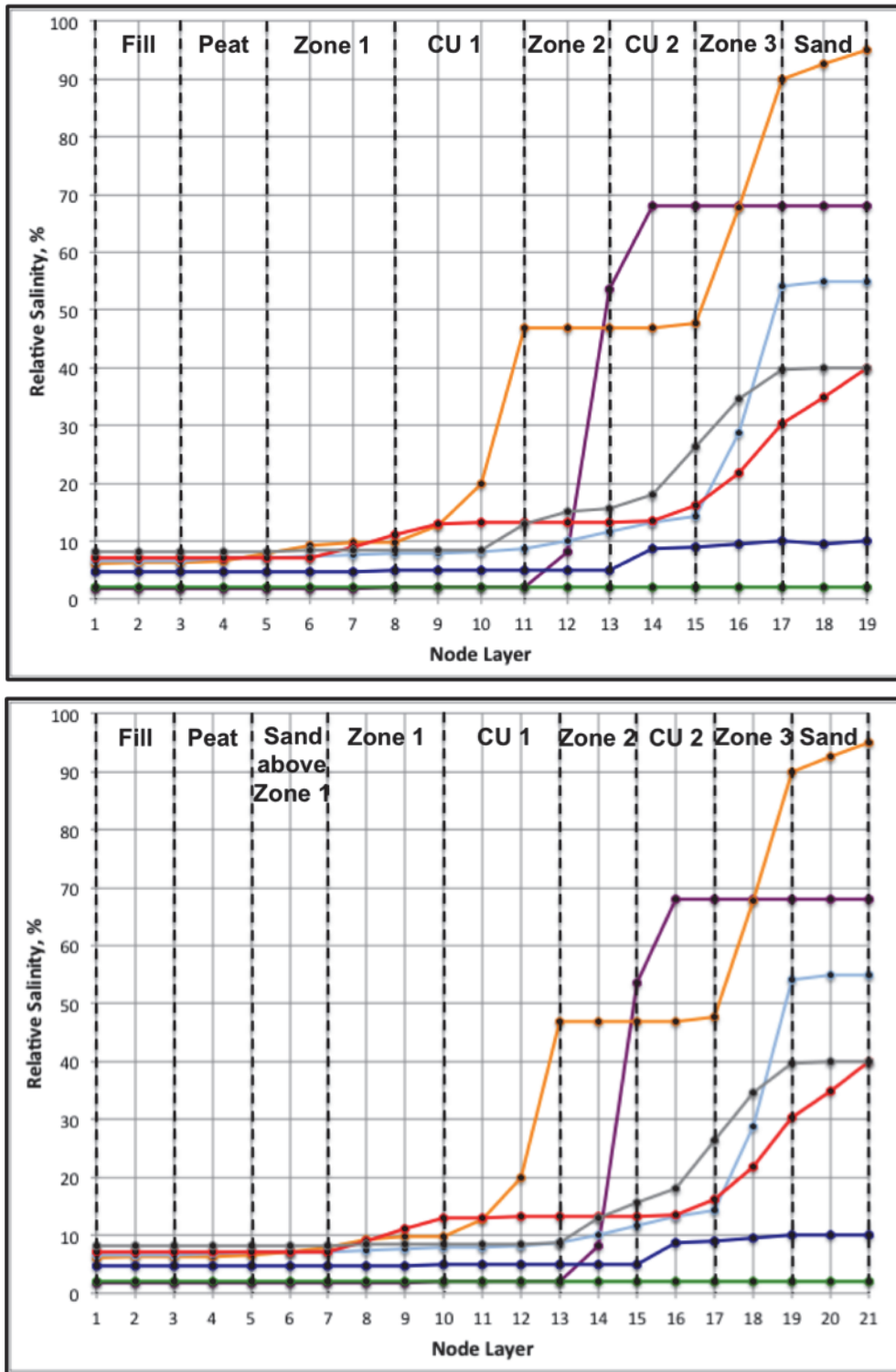
Figure 6. Geology-based interpolation using 19 (top) and 21 (bottom) geologic break points.
