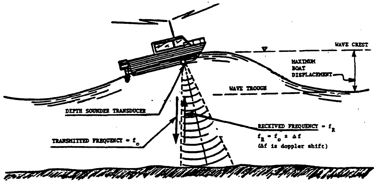
Figure 2. Doppler vertical motion detection principle
