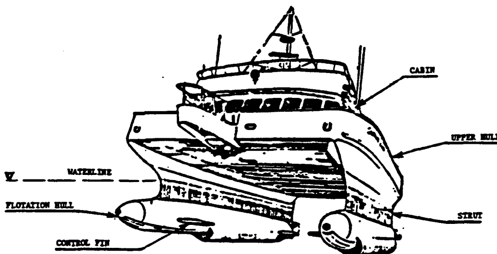
Figure 3. Small waterplane area twin hull (SWATH)
