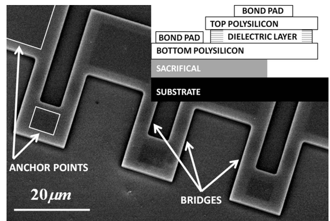
FIG. 1. A scanning electron micrograph showing the six-bridge structure common to p-sox-p and p-sn-p devices (image is of p-sox-p device). Layer thicknesses are: ( p_{\text{bottom-sox-p-top}} ) 277 nm-53 nm-303 nm; ( p_{\text{bottom-sn-p-top}} ) 280 nm-50 nm-106 nm. Contrast is altered to highlight the undercut at the anchor points, which are highlighted in white as are three of the six bridges. The gold bond pads are not shown. Inset: a side-view schematic of the layer stack.
