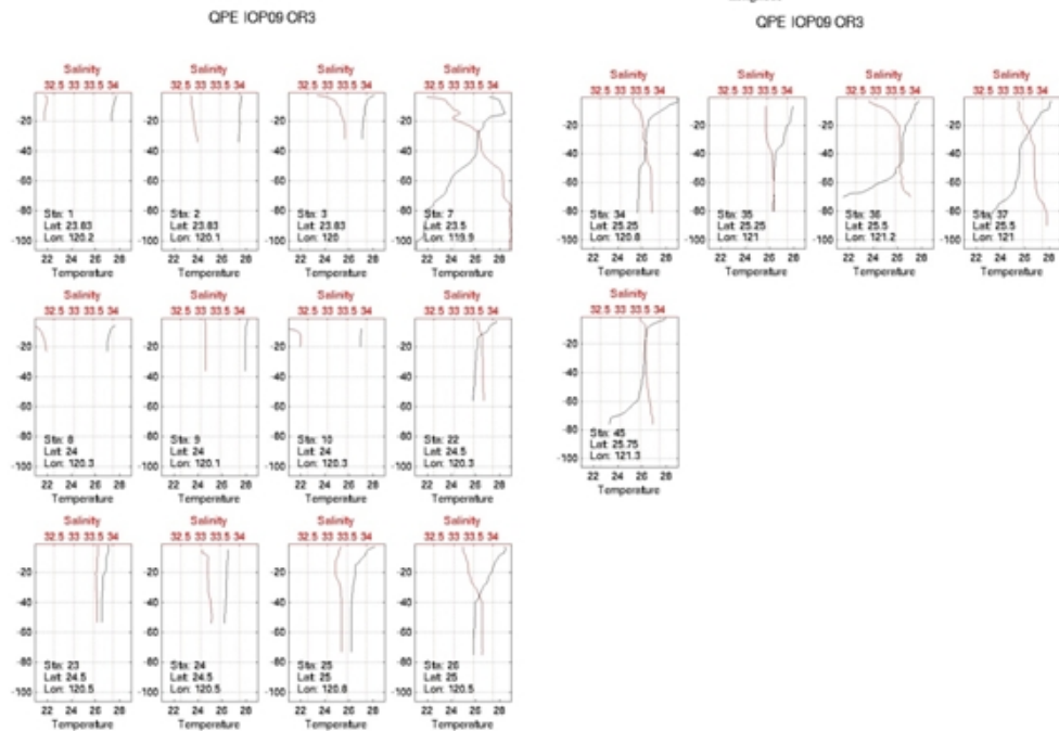
Figure 3-6: Salinity profiles and locations of low salinity observations in the wake of Typhoon Morakot. (Leslie, 2012)
