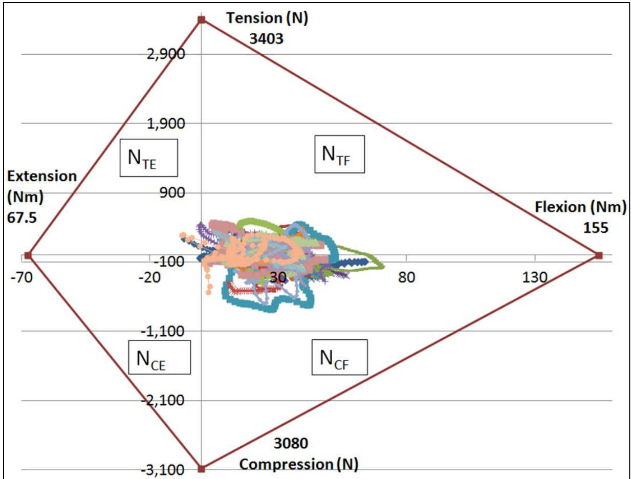
Figure 11. Plot of Human N_{ij} Values and Intercepts (8 G Acceleration with 2 kg HMD)
