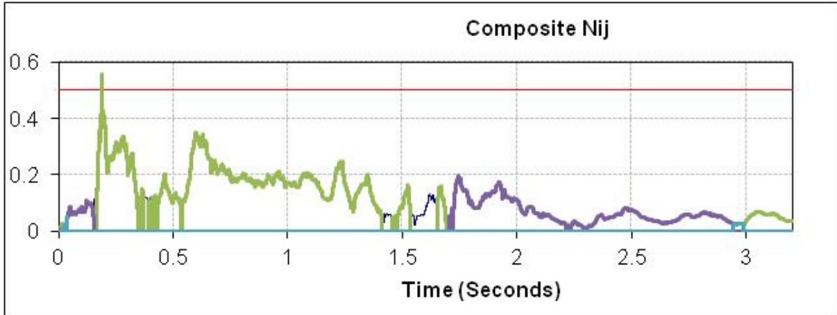
Figure 7. Example Sled Test Upper Neck ATD Data Compared to Nij Limit of 0.5
