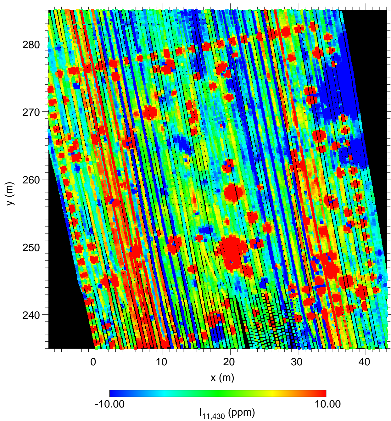
Figure 16 – Anomaly image of the 11,430 Hz in-phase response at the APG Blind Grid
