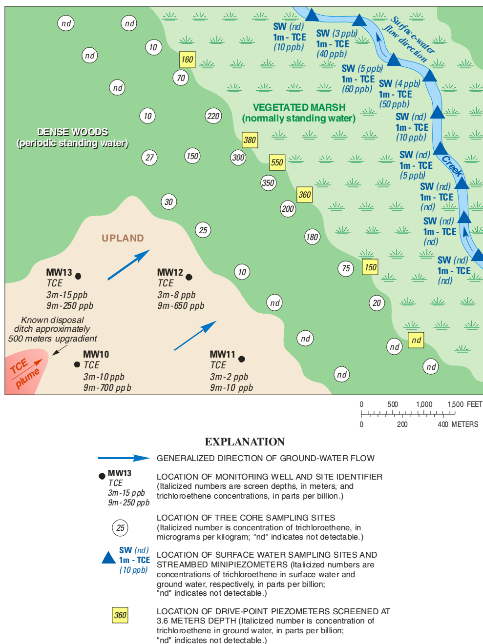
Figure 16. Schematic of a hypothetical site with a trichloroethene ground-water contamination plume showing concentrations of trichloroethene in ground water (3.6-meter depth using drive-point piezometers) from third phase of chlorinated solvent natural attenuation reconnaissance activity.
