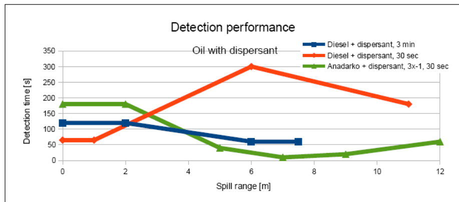
Figure C-3. WBMS detection with dispersant.
