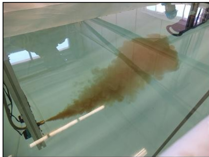
Figure A-6. Test plume being created.
