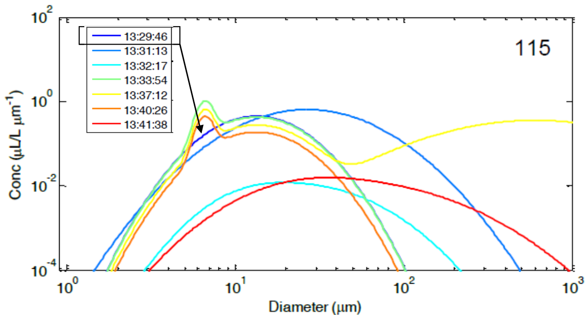
Figure 34. WINDOW droplet size concentration from Test #115.
