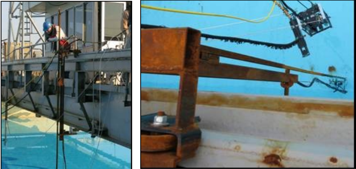
Figure 5. Trolley on Ohmsett main bridge.
