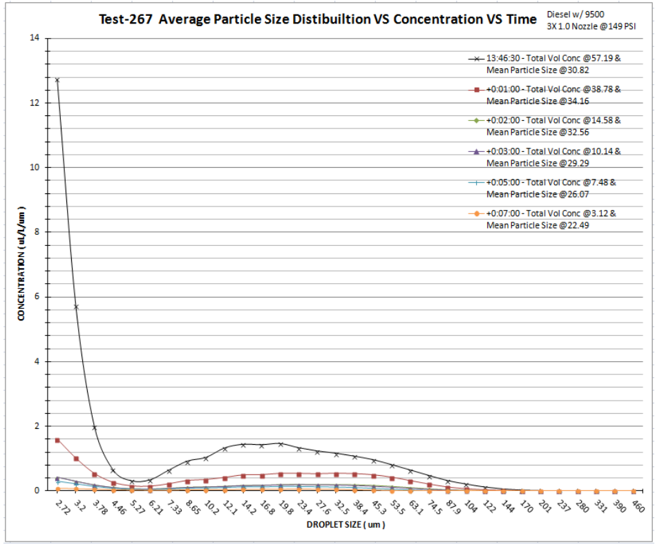
Figure D-2. WBMS Test #267 average particle size distribution.
