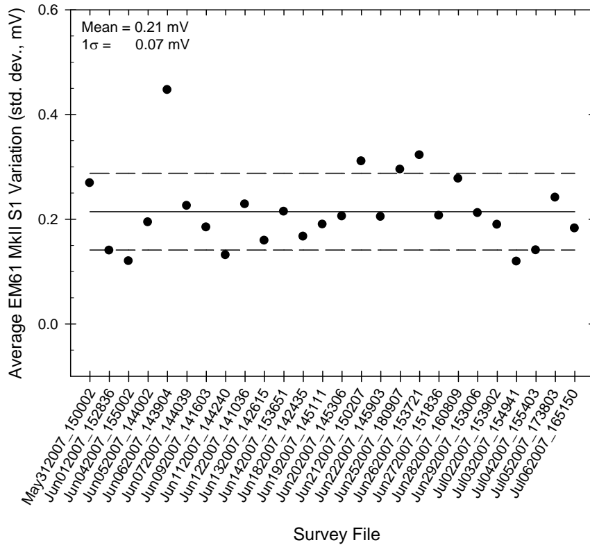
Figure 3-20 – Overall variation of the MP EM61 MkII system (S1). The horizontal axis is survey file number. The solid line represents the aggregate average sensor variation and the dashed lines represent a 1σ envelope.
