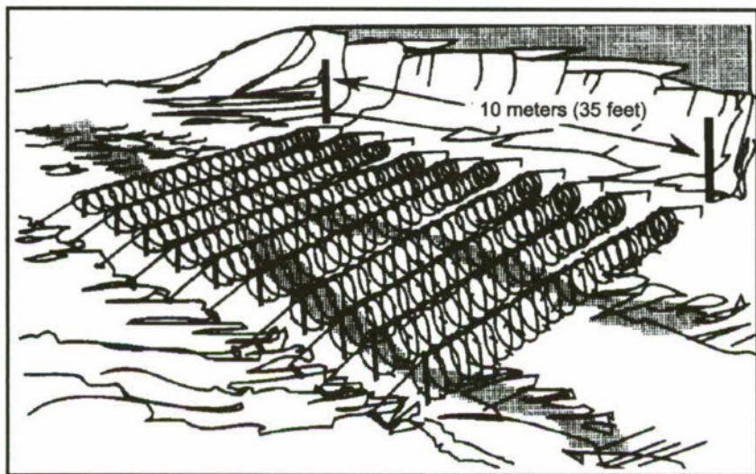
Figure C-4C. Concertina wire roadblock.
