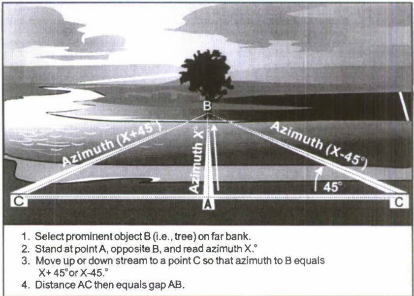
Figure 9-4. Measuring stream width with a compass.
