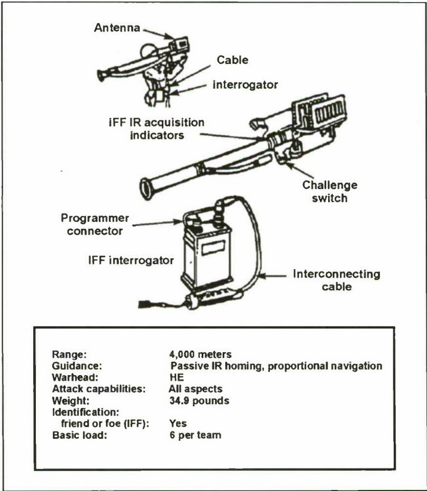
Figure 6-17. Stinger air defense system.
