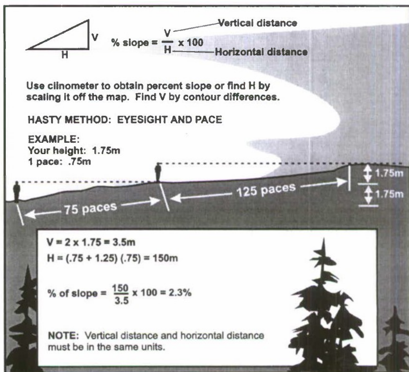
Figure 9-6. Slope computation (road gradient).
