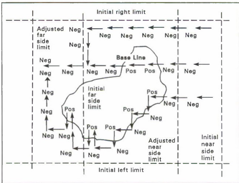
Figure B-4. Adjusting the limits of the contaminated area.
