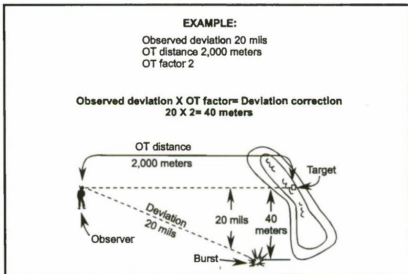
Figure 8-26. Converting mil deviation to deviation correction.
