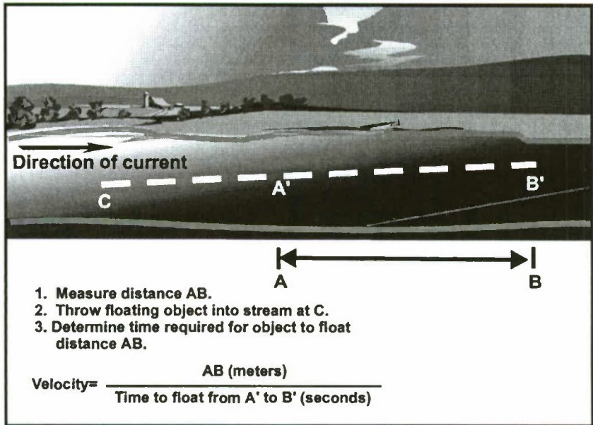
Figure 9-5. Measuring stream velocity.
