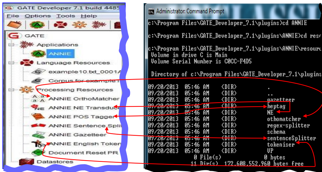
Figure 3. GUI and command line listings of ANNIE PRs.
