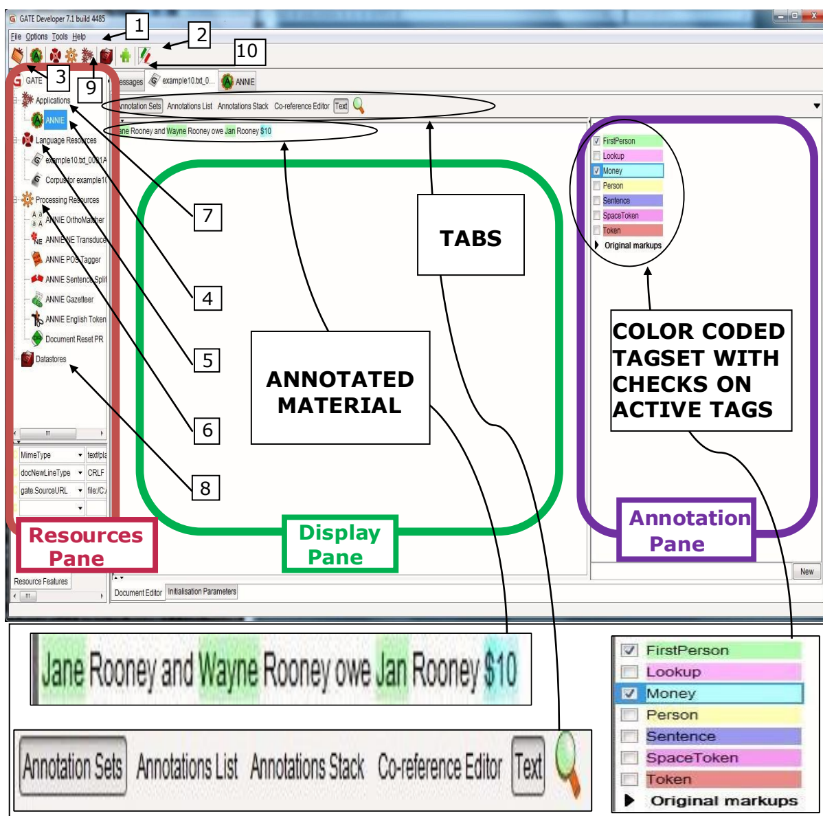
Figure 2. GATE Developer GUI.
