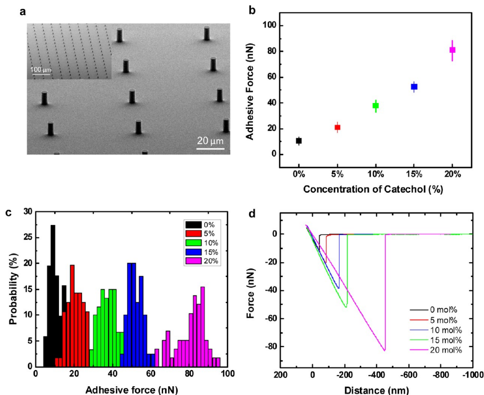
Figure 3. Measurement of adhesive force for fabricated microstructures based on catechol-functionalized polysiloxanes after deprotection. (a) SEM images of fabricated microstructures ( 5 \mu\text{m} diameter, 10 \mu\text{m} height, 2:1 aspect ratio). (b) Plot of adhesive force vs concentration of catechol units in the starting polysiloxane. (c) Histogram of adhesive force vs concentration of catechol units in the starting polysiloxane. (d) Representative force–distance curves of fabricated microstructures incorporating different concentrations of catechol from 0 to 20 mol %.
