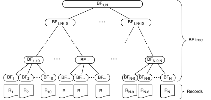
Let (R_1, \dots, R_n) be the overall database records. The Bloom filter BF_{a,b} contains all the keywords of records R_a, R_{a+1}, \dots, R_b .
