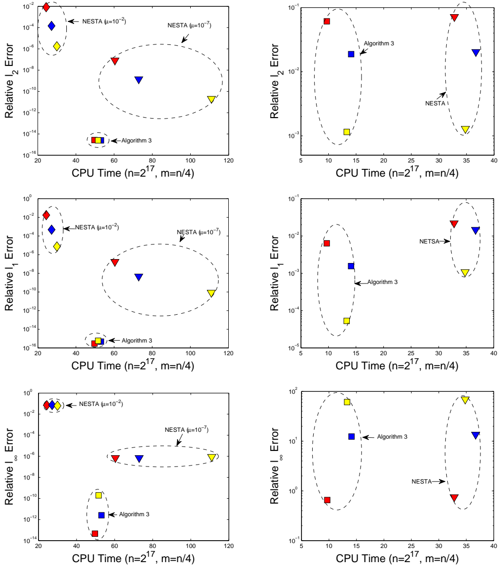
Figure 4.2: The relative l_1 , l_2 , and l_\infty errors (the vertical axis with base 10 logarithmic scale) versus the CPU time consumed (the horizontal axis) for (the left-column) the noise free case and (the right-column) the noise case. The colors ‘red’, ‘blue’, and ‘yellow’ represent the dynamic ranges of the tested signals with \theta being 1, 3, and 5, respectively.
