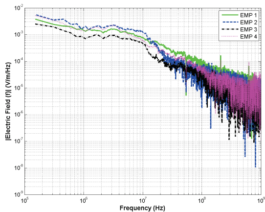
Figure 8: Various measured EM pulse frequencies generated by the PS-6 pulser with various switch timing parameters.
