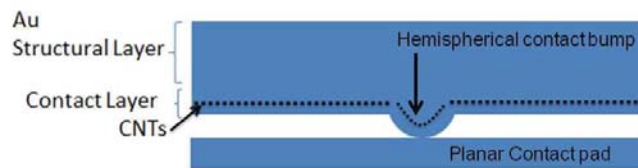
Figure 3.5: Example cross-section of a Au-CNT contact device.
