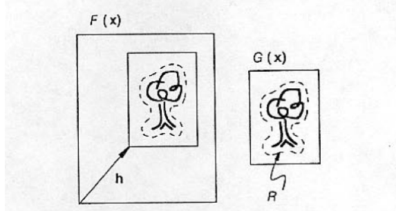
Figure 9: From the original Lucas-Kanade paper (1981): “We wish to find the disparity vector h which minimizes some measure of the difference between F(x + h) and G(x) for x in some region of interest R ”.
