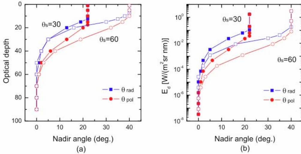
Figure 1. Movement of \theta_{rad} and \theta_{pol} as the optical depth increases and the downward plane irradiance decreases, in a coupled atmosphere-ocean system. The Petzold phase function was used for the ocean, and a single scattering albedo \omega_0 = 0.9 was assumed. Results for two solar zenith angles \theta_s = 30^\circ (curves with solid symbols) and \theta_s = 60^\circ (curves with open symbols) are shown. This figure shows that the radiance (blue curves) reaches its asymptotic form more quickly than the degree of polarization (blue curves) does. The asymptotic region for the radiance is reached at optical depth of 60, while the asymptotic region for the degree of polarization is reached at optical depth of 70. The curve on the right shows the actual peak radiance relative to a 1 \text{ W}/(\text{m}^2 \text{ nm}) source at the top of the atmosphere
