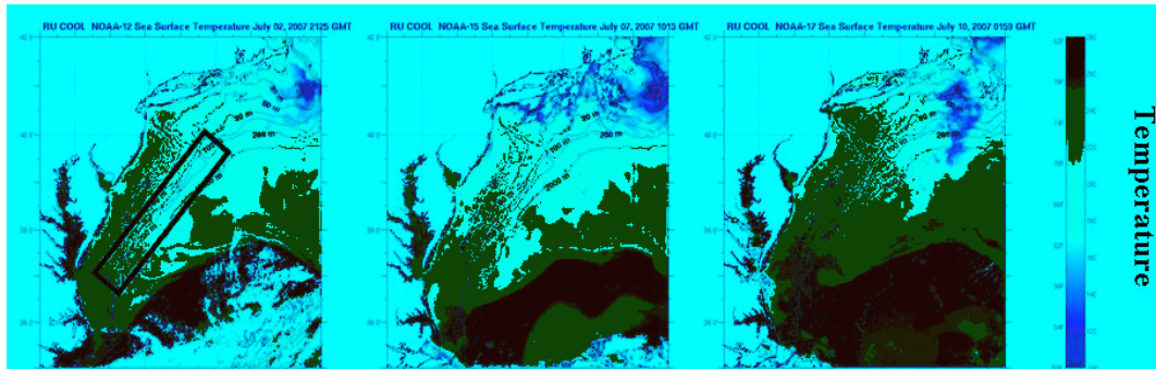
Figure 1. Sea surface temperature maps of the Mid-Atlantic Bight during the PIMMS Spritz cruise. The ship sampling was concentrated in the bold line box. Major hydrography was influenced by the interplay between 1) offshore forcing from Gulf Stream and associated meanders as well as 2) nearshore upwelling. Dark blue areas in the Grand Bank region reflects cloud contamination which was associated with weather patterns that provided challenging conditions.
