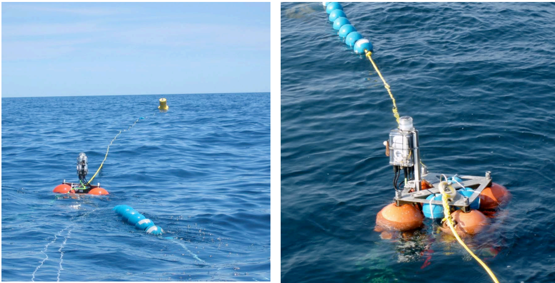
Figure 5. PIMMS mooring deployed off NJ in July 2007 showing the surface floats (blue), battery buoy (orange), and mooring buoy (yellow).
