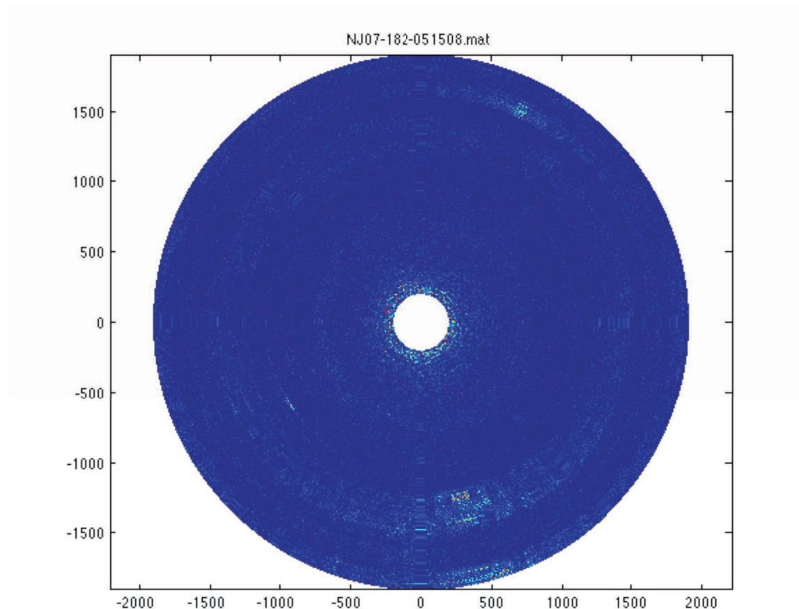
Figure 6: Backscatter image of the horizontal waveguide. Several small areas of increased backscatter are attributed to fish schools moving across the image. This image is taken from a time series of backscatter images recorded using the PIMMS mooring over a 24 hour period.
