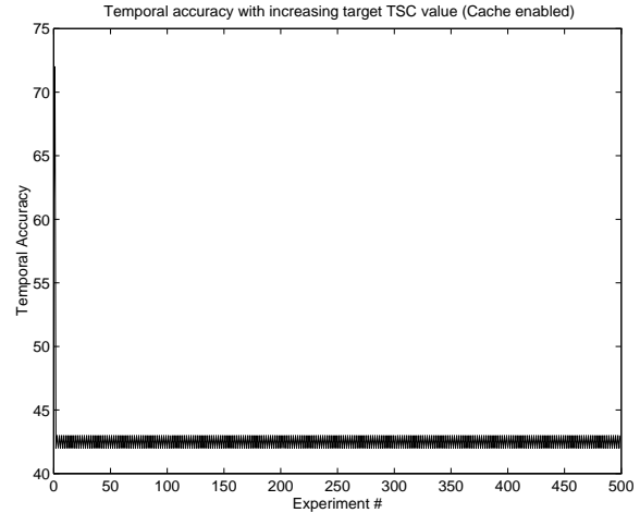
Figure 8: Temporal Accuracy for increasing Target TSC values with lookup table based delay loop
