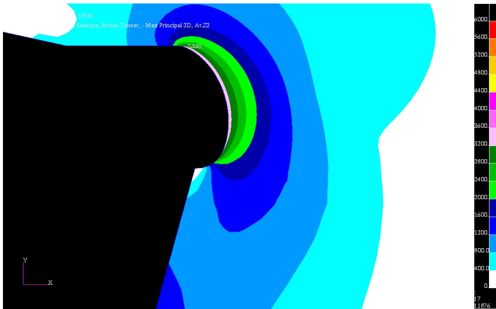
Figure 2: Shape and stress distribution for the shallow rework (peak stress concentration reduced by 45%)
