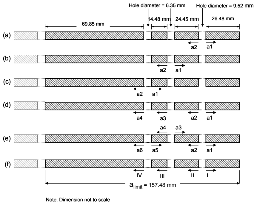
Figure 5 Crack scenarios analysed for MSD (cases a, b, c, d, e) and the phase-by-phase approach (case f)
