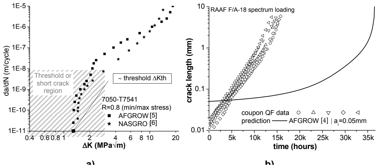
Figure. 1: AA7050 crack growth a) da/dN v \Delta K data and b) analytical LEM prediction of coupon(QF - quantitative fractography) test results with RAAF F/A-18 Hornet wing root bending moment spectrum.
