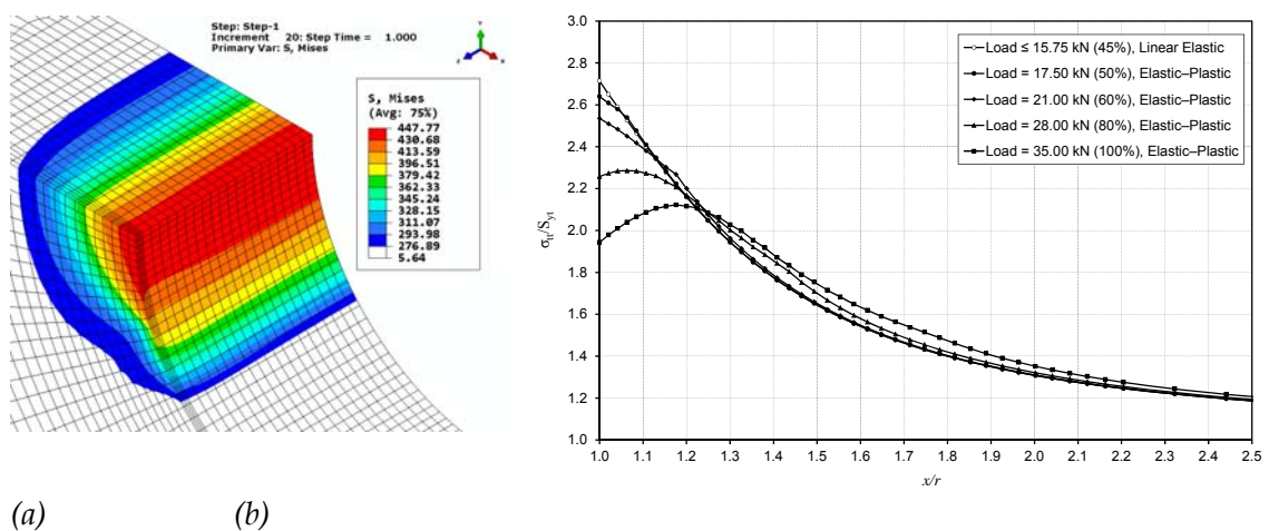
Figure 3: (a) Von Mises stress in the plastic zone around the hole boundary in the coupon at the maximum applied load, P = 35 \text{ kN} . (b) Normalised tangential stress as a function of radial distance away from the edge of the hole at the \theta = 0^\circ location at the plate mid-plane.
