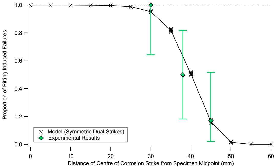
Figure 3: Proportion of experimental and predicted failures due to pitting for single and dual symmetric corrosion strikes vs. distance from the midpoint of the specimen. \sigma_{max} = 380 MPa, R = 0.1 and each data point represents 5,000 replicates.
