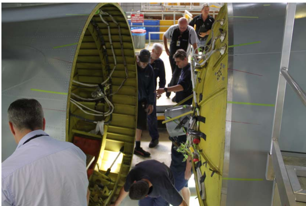
Figure 2: Empennage removal for FS1117 refurbishment
