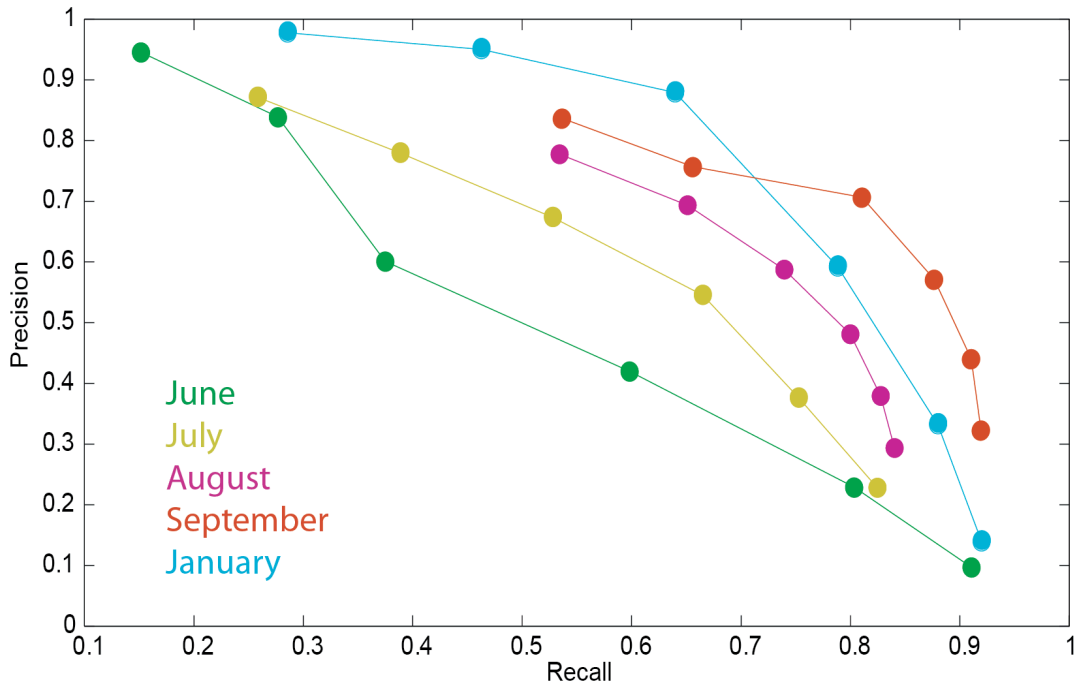
Figure 1 - Seasonal variation in the precision and recall of Blue whale B call detections from an instrument in the Southern California Bight ( 118.57^{\circ} W , 32.37^{\circ} N ) during the 2011 field season.
