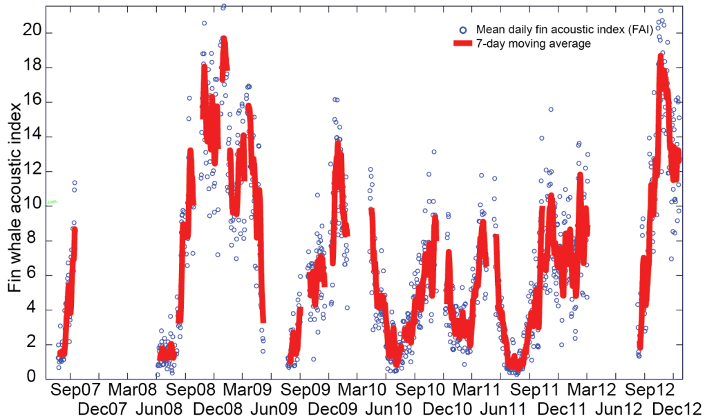
Figure 2 - Acoustic power index denoting presence of calling fin whales over a five year period in the Southern California Bight ( 119.17^{\circ} W , 32.84^{\circ} N ). A seven day moving average is plotted over the daily indices.
