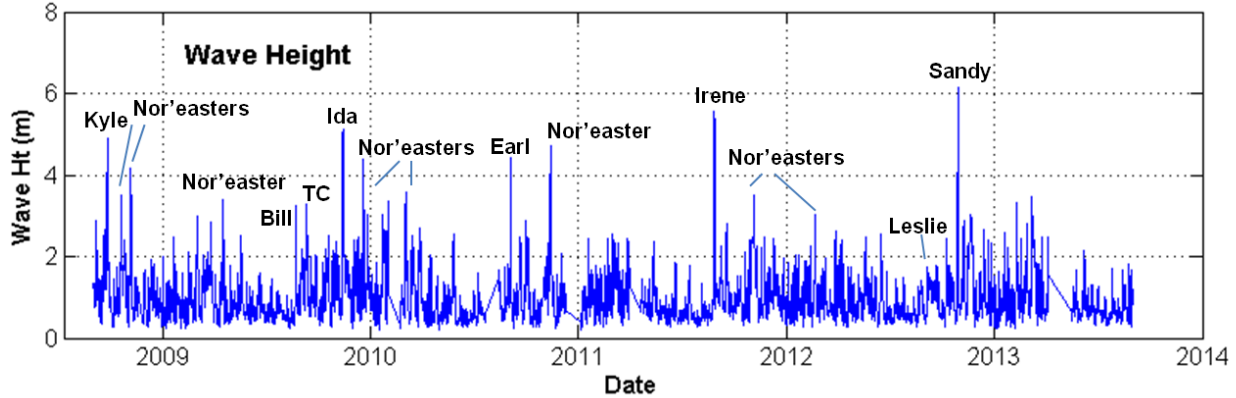
Figure 2. Sample wave height climatology (Aug 2008 – Sep 2013) from FRF 18-m Waverider station.
