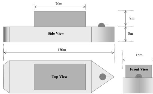
Figure 12: Ship geometry
