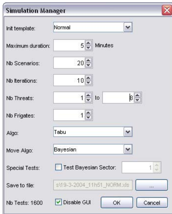
Figure B.7: Simulation manager panel
