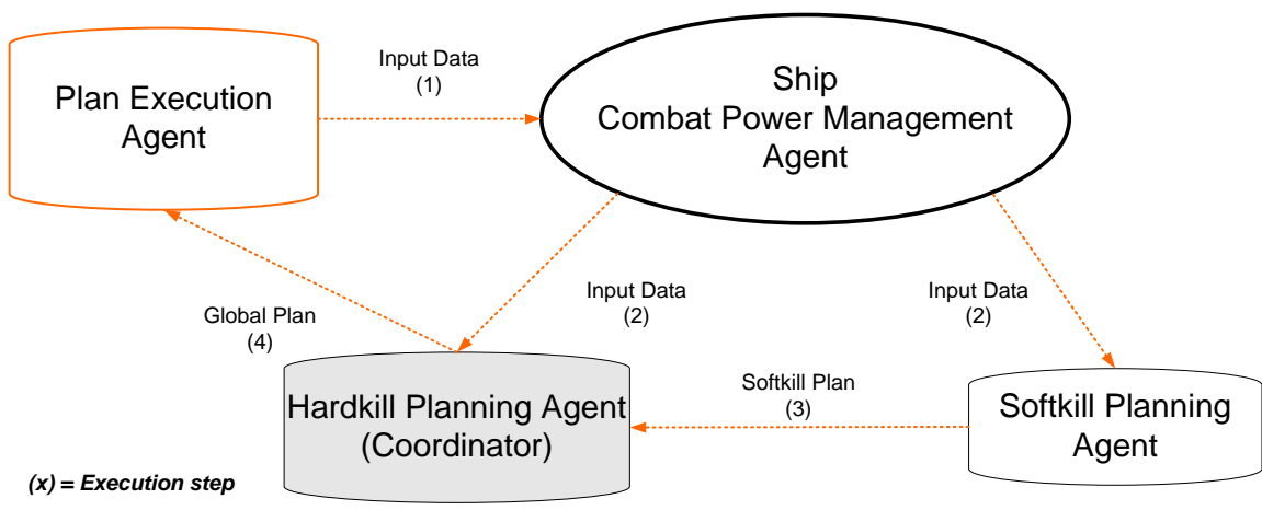
Figure 3: Data flows in Hardkill Agent as a coordinator planning process
