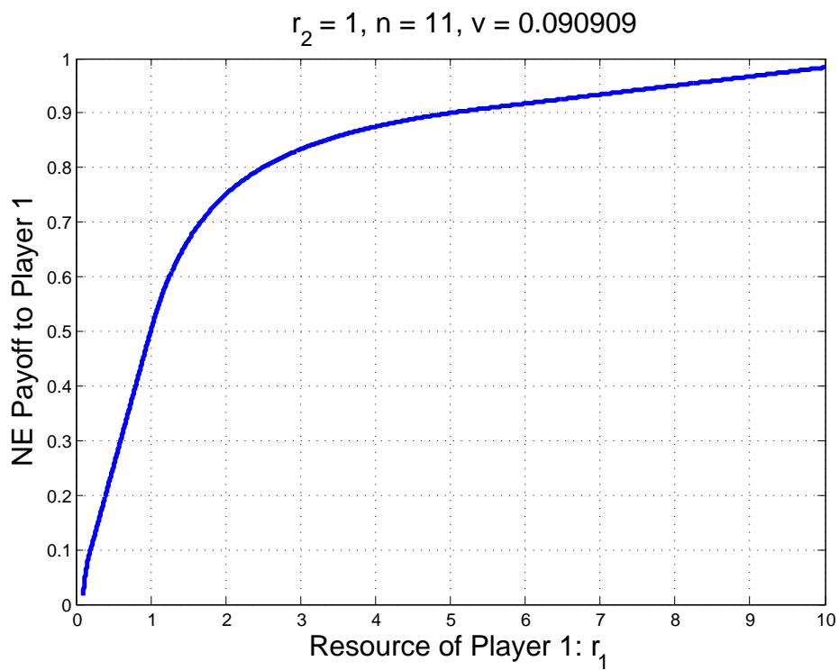
Figure 1: For a fixed resource r_2 of Player 2, the payoff to Player 1 is concave function of its endowment of resources r_1 .
